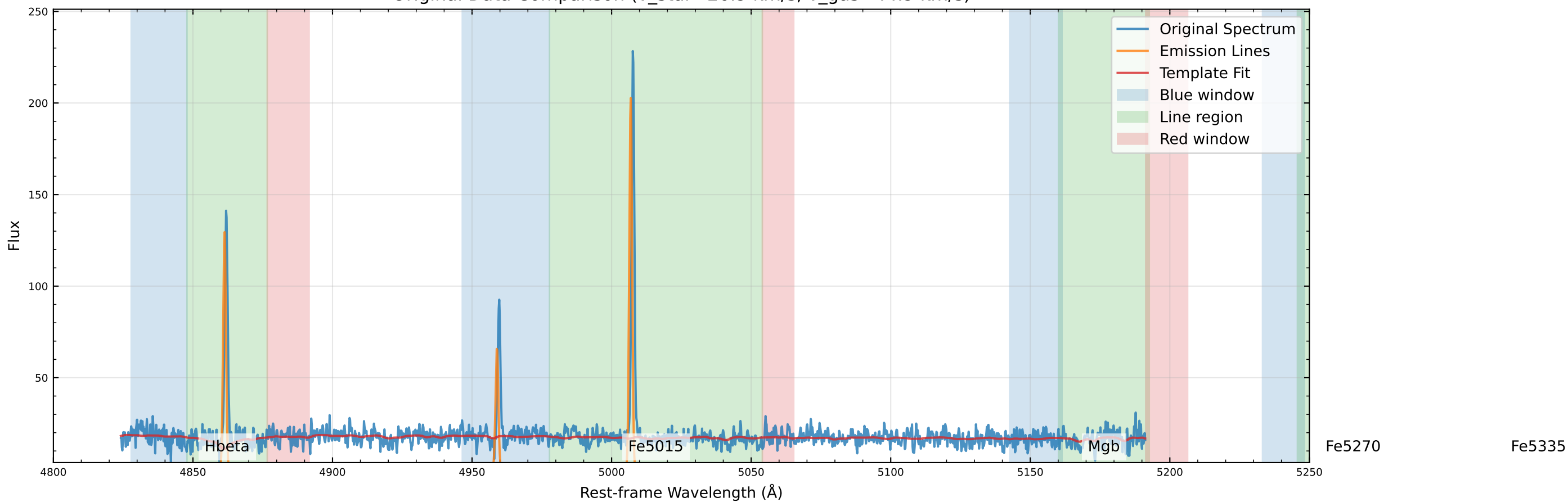
Original Data Comparison (v_star=26.9 km/s, v_gas=44.9 km/s)
