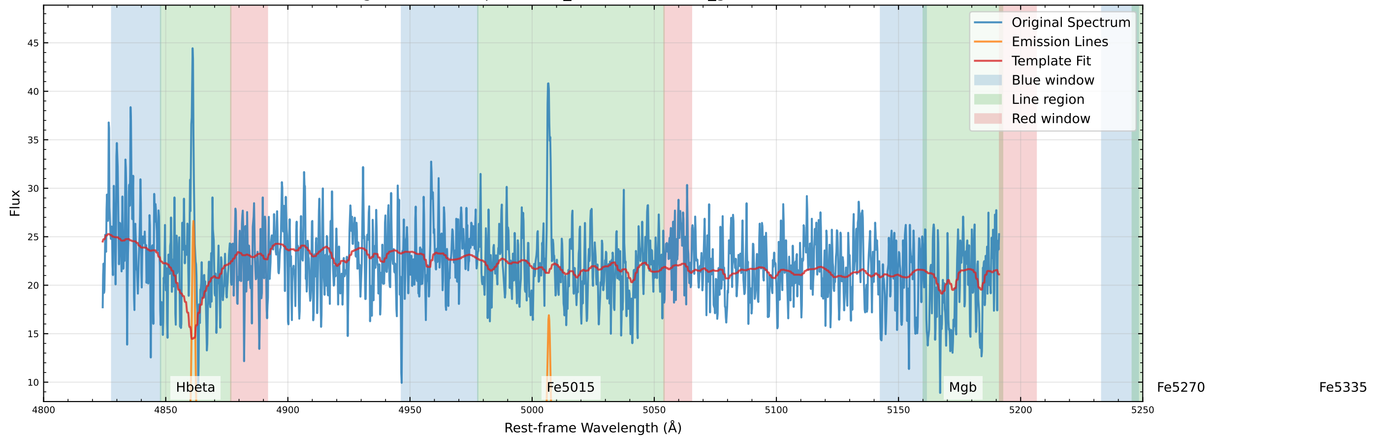
Original Data Comparison (v_star=-6.3 km/s, v_gas=-16.2 km/s)
