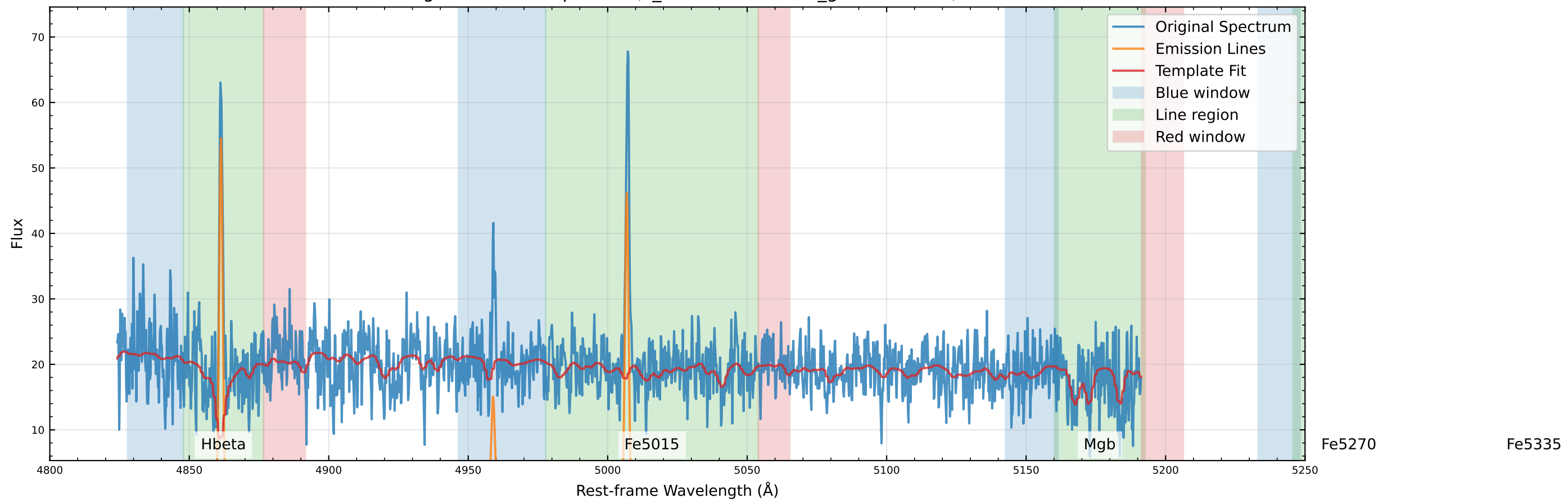
Original Data Comparison (v_star=-2.4 km/s, v_gas=8.8 km/s)
