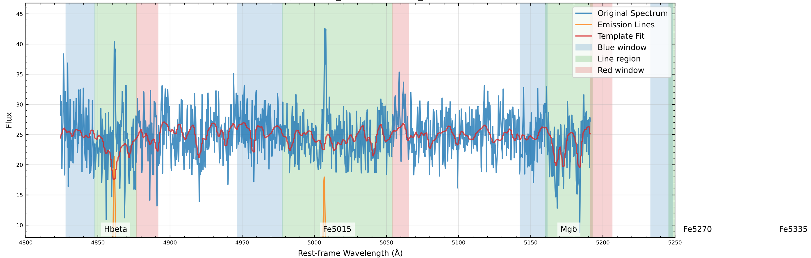
Original Data Comparison (v_star=9.5 km/s, v_gas=27.2 km/s)
