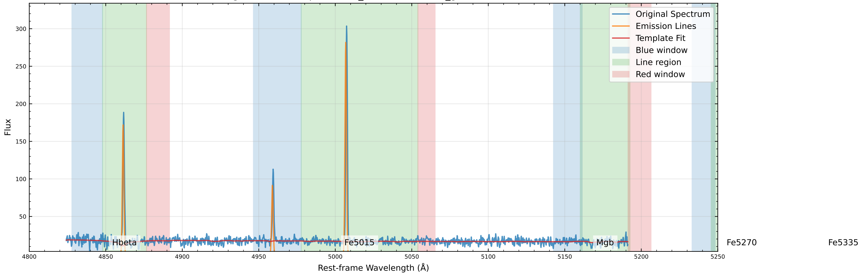
Original Data Comparison (v_star=4.6 km/s, v_gas=31.8 km/s)
