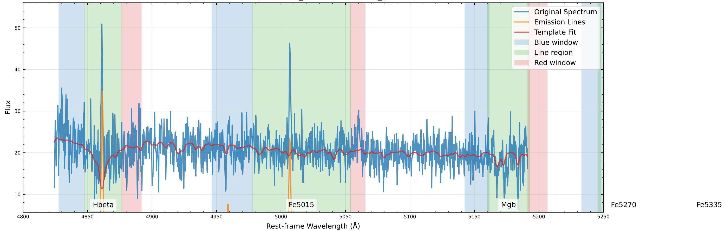
Original Data Comparison (v_star=21.6 km/s, v_gas=-3.3 km/s)
