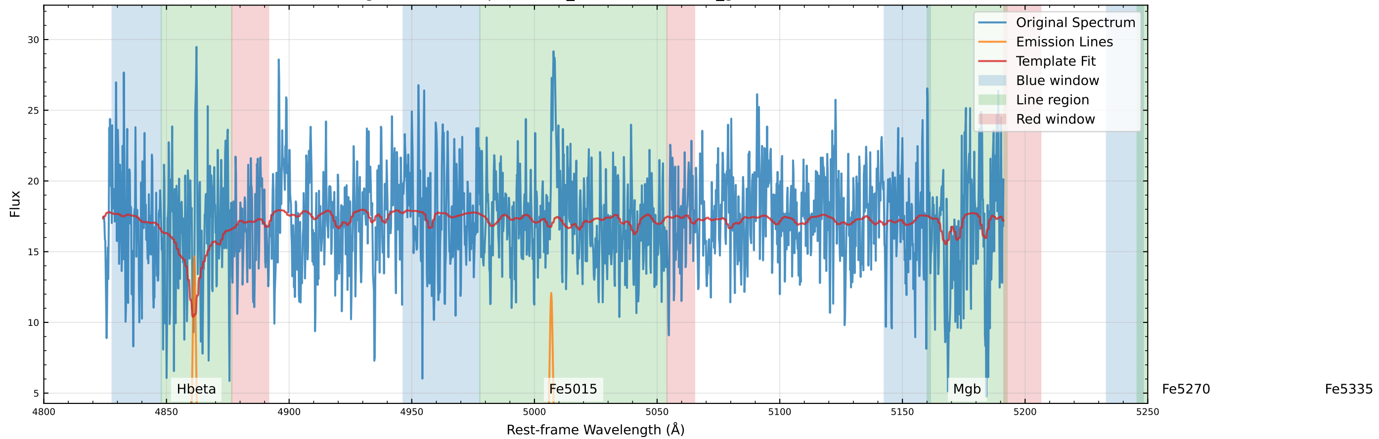
Original Data Comparison (v_star=60.1 km/s, v_gas=57.2 km/s)
