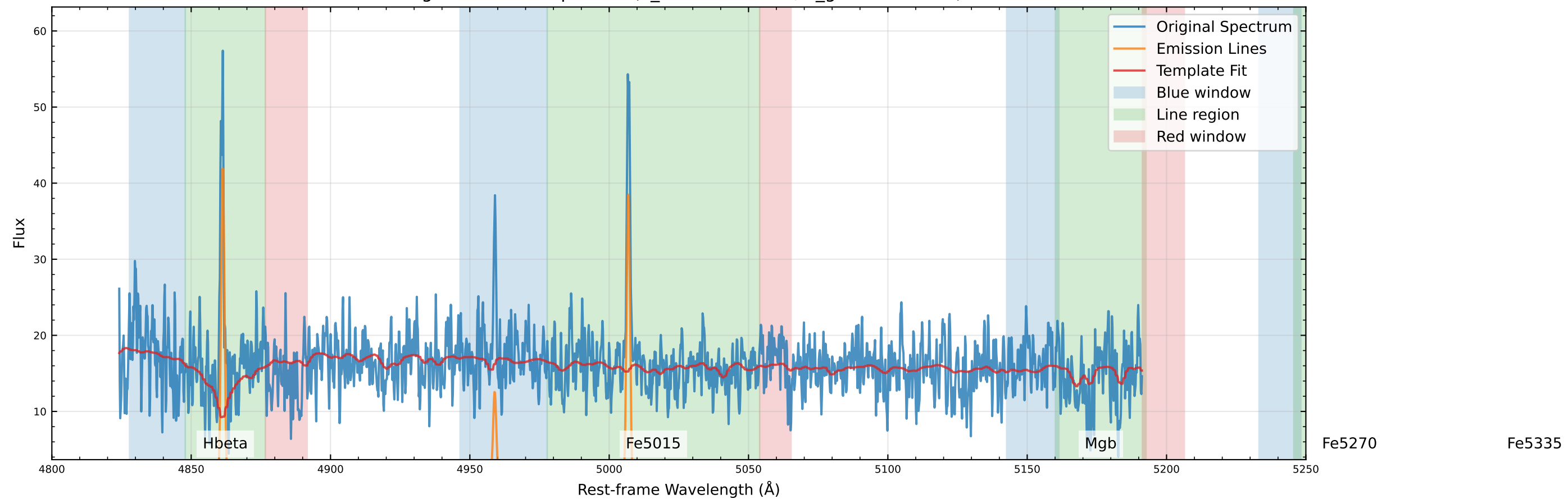
Original Data Comparison (v_star=-7.1 km/s, v_gas=-6.8 km/s)
