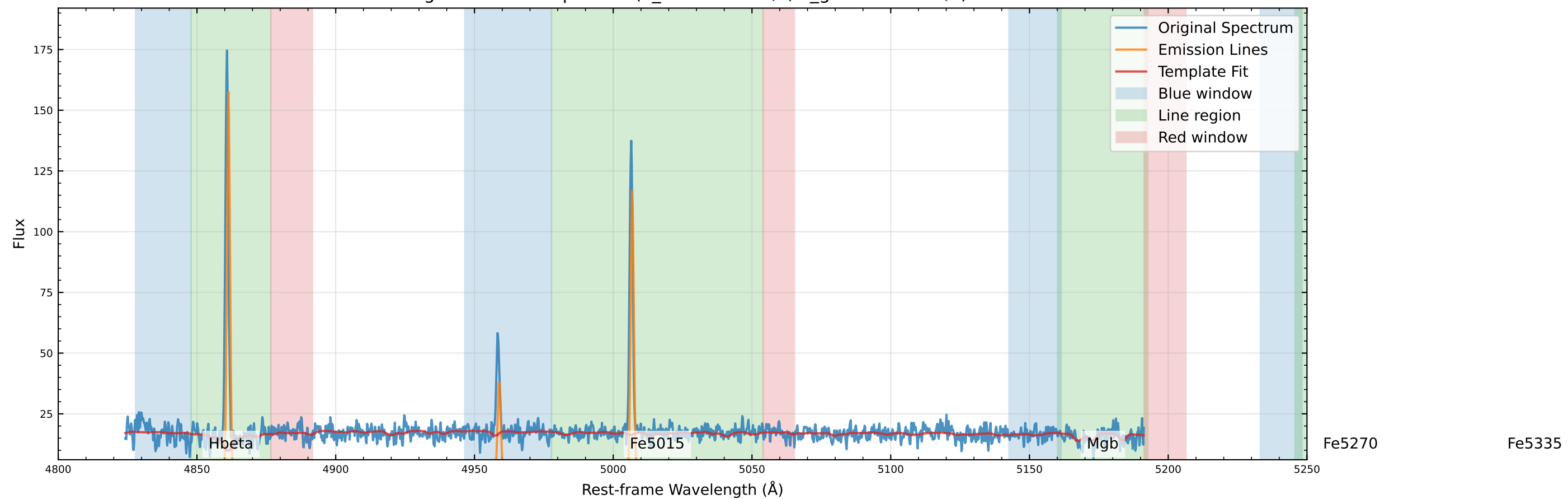
Original Data Comparison (v_star=9.6 km/s, v_gas=-30.9 km/s)
