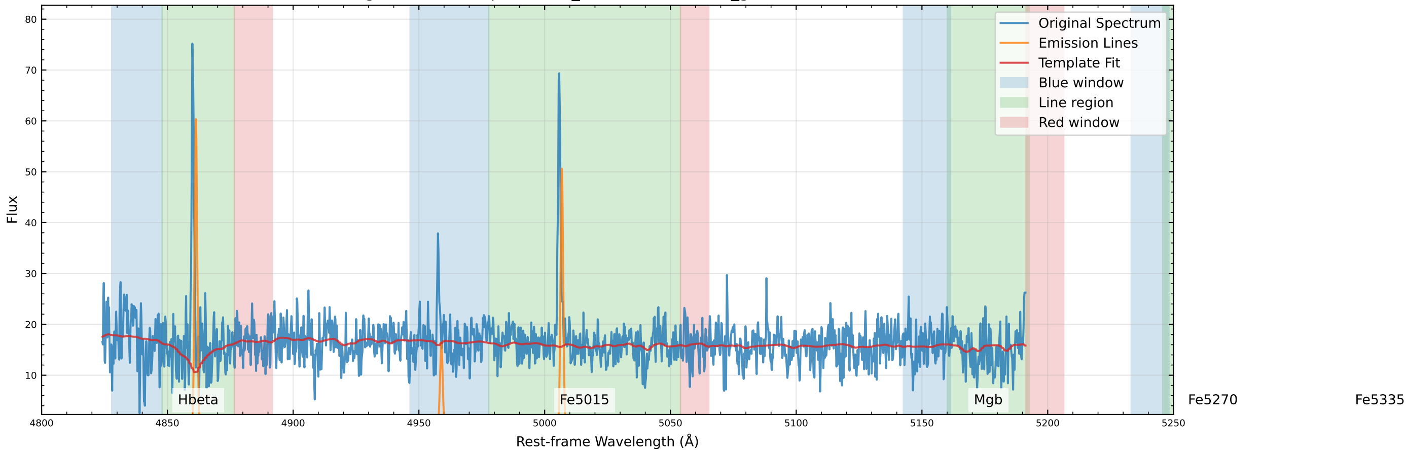
Original Data Comparison (v_star=-58.3 km/s, v_gas=-70.7 km/s)
