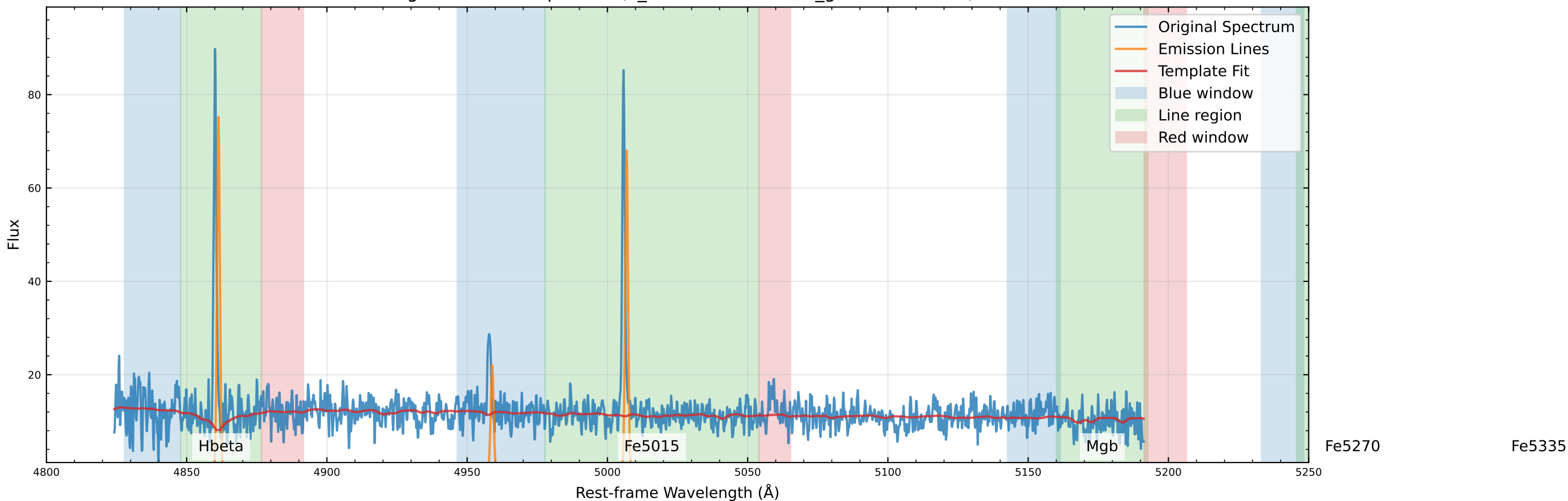
Original Data Comparison (v_star=-76.9 km/s, v_gas=-70.1 km/s)
