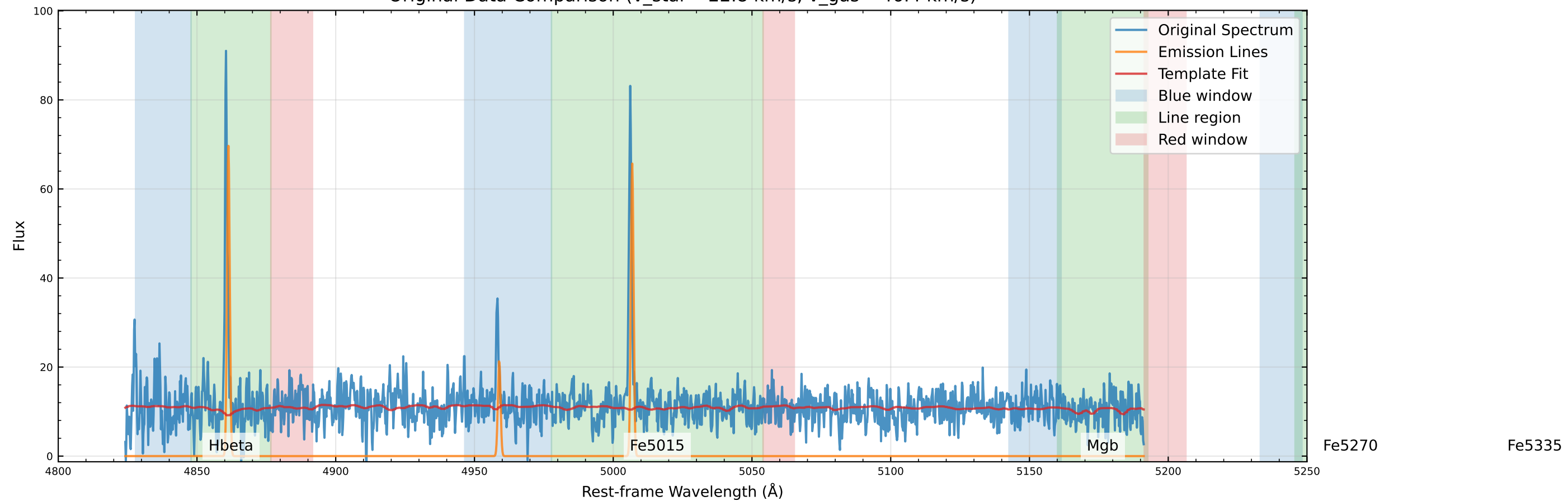
Original Data Comparison (v_star=-22.8 km/s, v_gas=-46.4 km/s)
