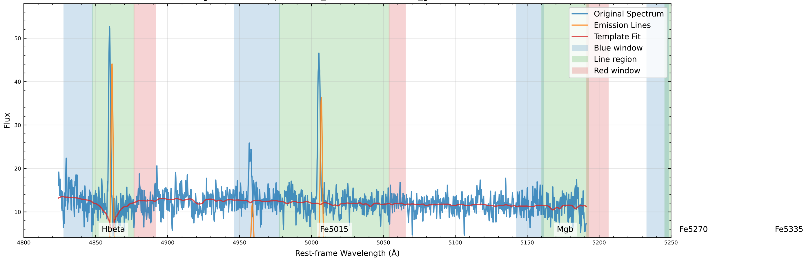
Original Data Comparison (v_star=-107.3 km/s, v_gas=-102.1 km/s)
