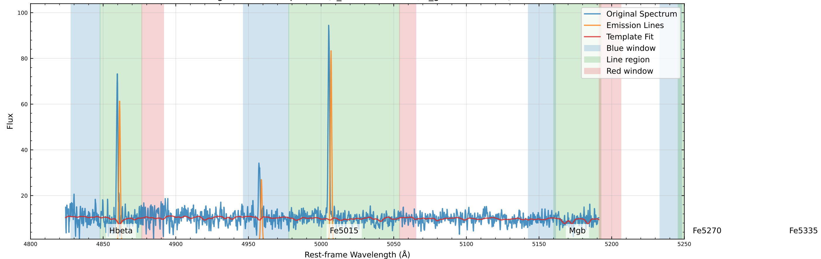
Original Data Comparison (v_star=-85.1 km/s, v_gas=-93.7 km/s)
