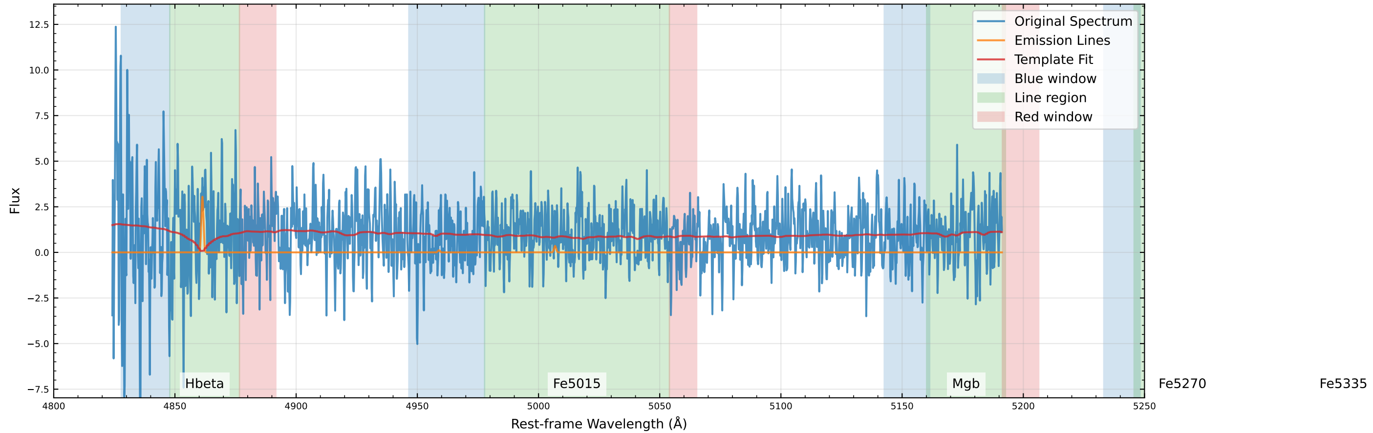
Original Data Comparison (v_star=-210.4 km/s, v_gas=-238.3 km/s)
