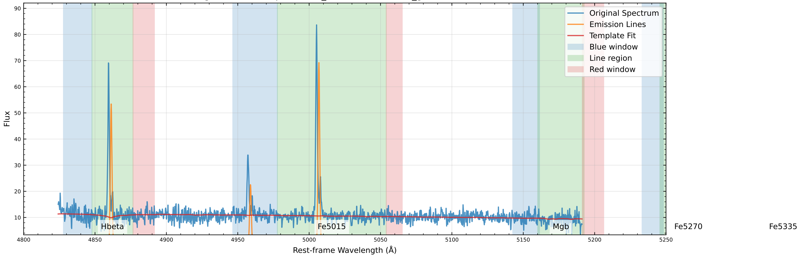
Original Data Comparison (v_star=-96.2 km/s, v_gas=-103.5 km/s)
