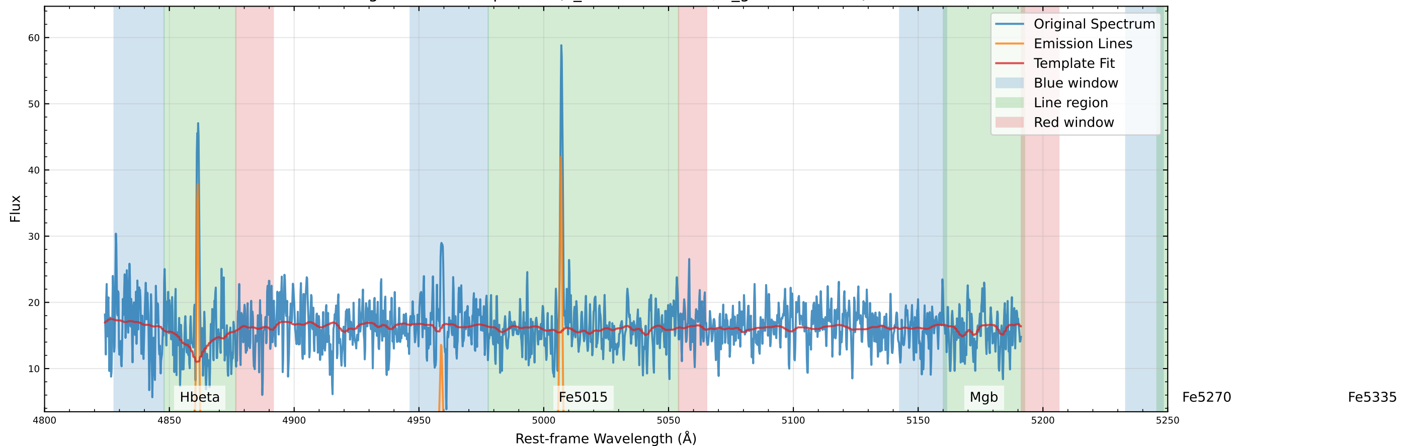
Original Data Comparison (v_star=-28.8 km/s, v_gas=11.9 km/s)
