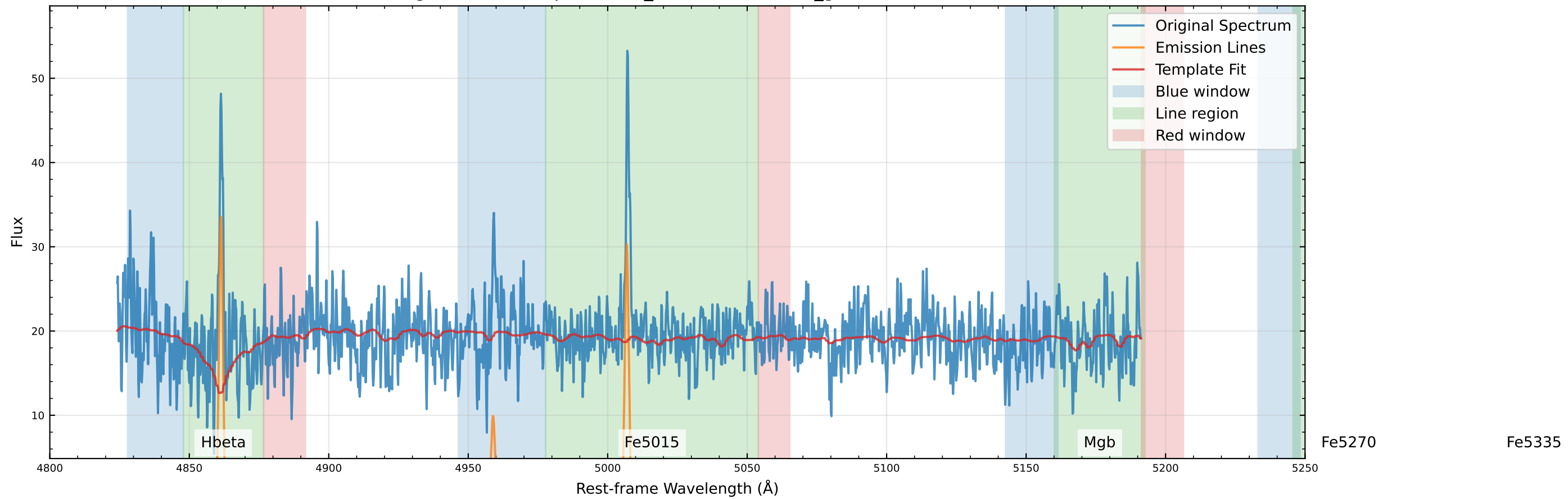
Original Data Comparison (v_star=14.0 km/s, v_gas=13.3 km/s)
