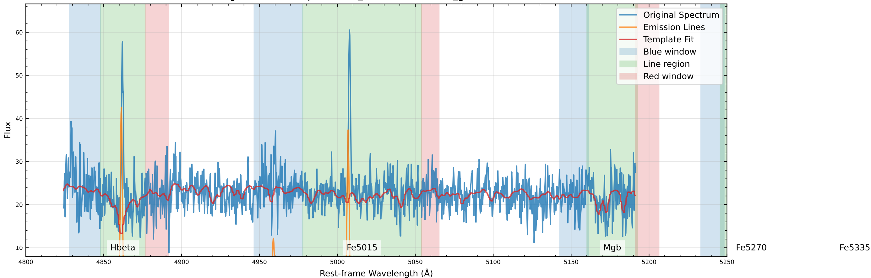
Original Data Comparison (v_star=40.9 km/s, v_gas=48.4 km/s)
