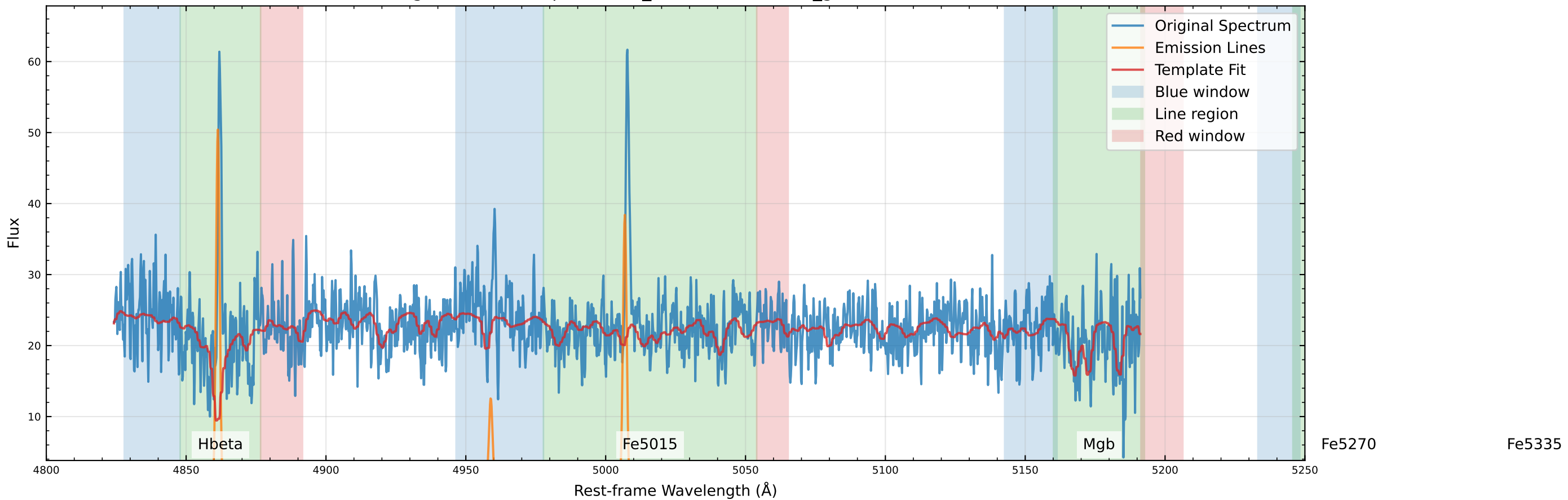
Original Data Comparison (v_star=45.2 km/s, v_gas=50.0 km/s)
