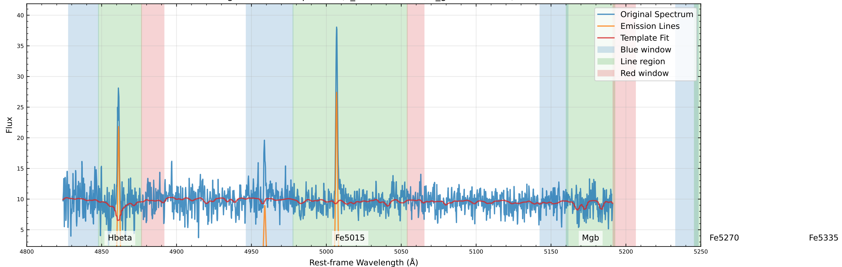
Original Data Comparison (v_star=7.0 km/s, v_gas=-1.5 km/s)
