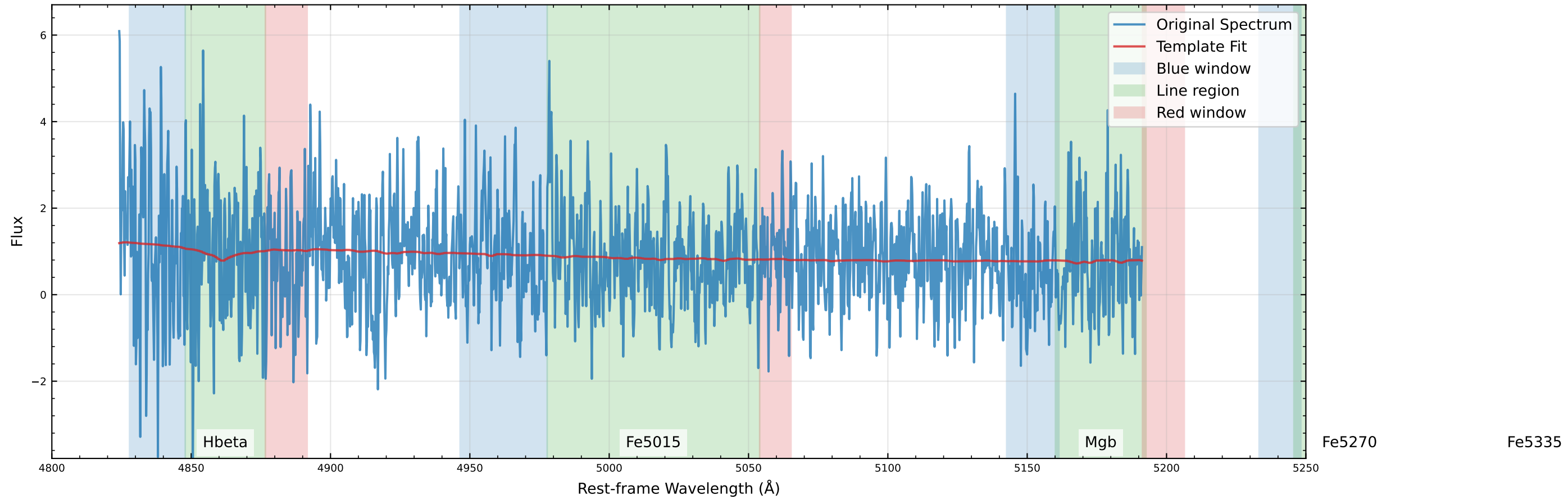
Original Data Comparison (v_star=-16.3 km/s)
