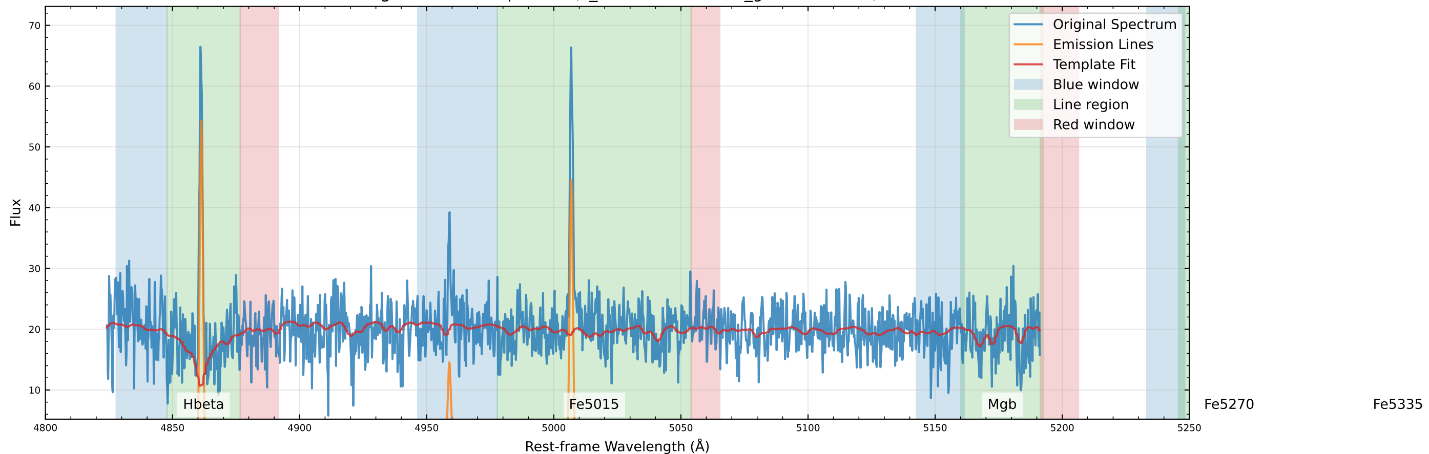
Original Data Comparison (v_star=27.5 km/s, v_gas=-4.1 km/s)
