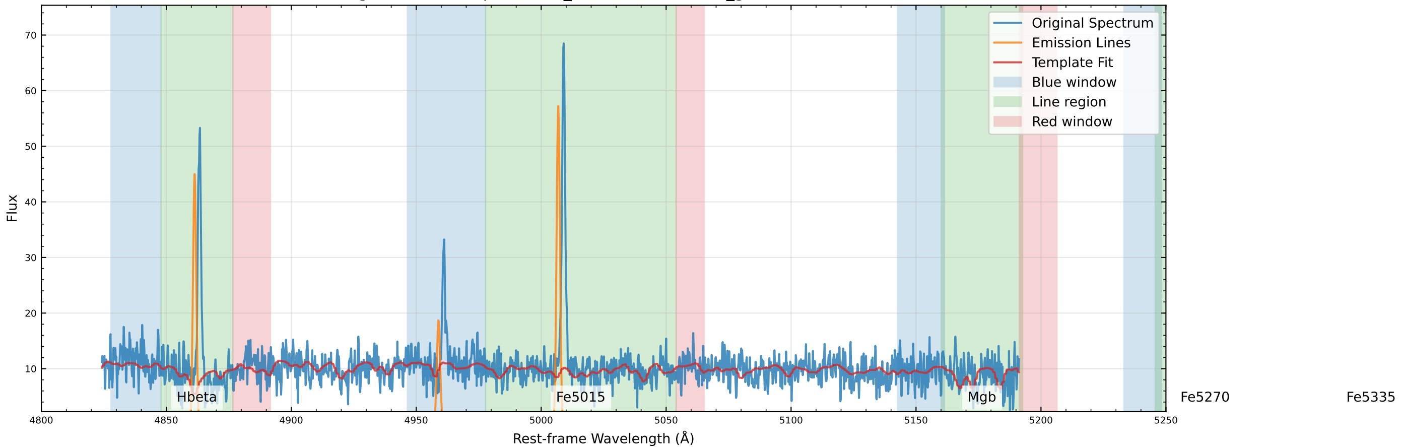
Original Data Comparison (v_star=117.4 km/s, v_gas=124.9 km/s)
