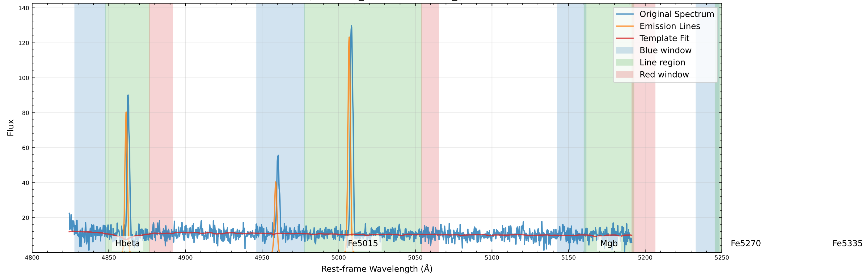
Original Data Comparison (v_star=38.8 km/s, v_gas=91.8 km/s)
