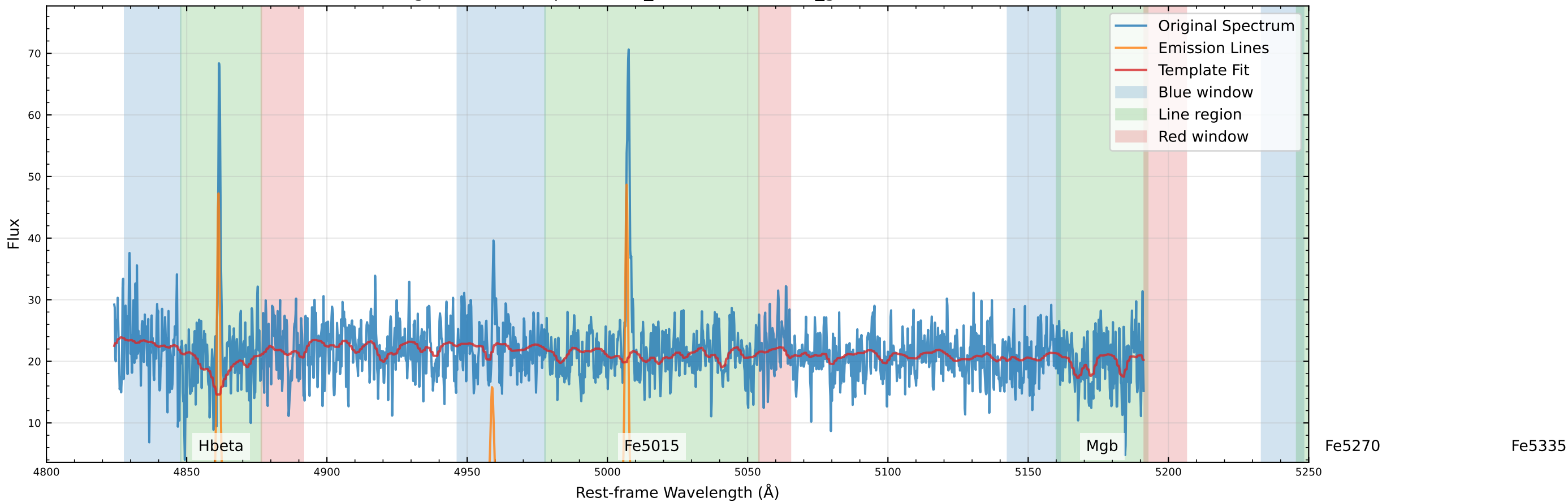
Original Data Comparison (v_star=21.0 km/s, v_gas=27.4 km/s)
