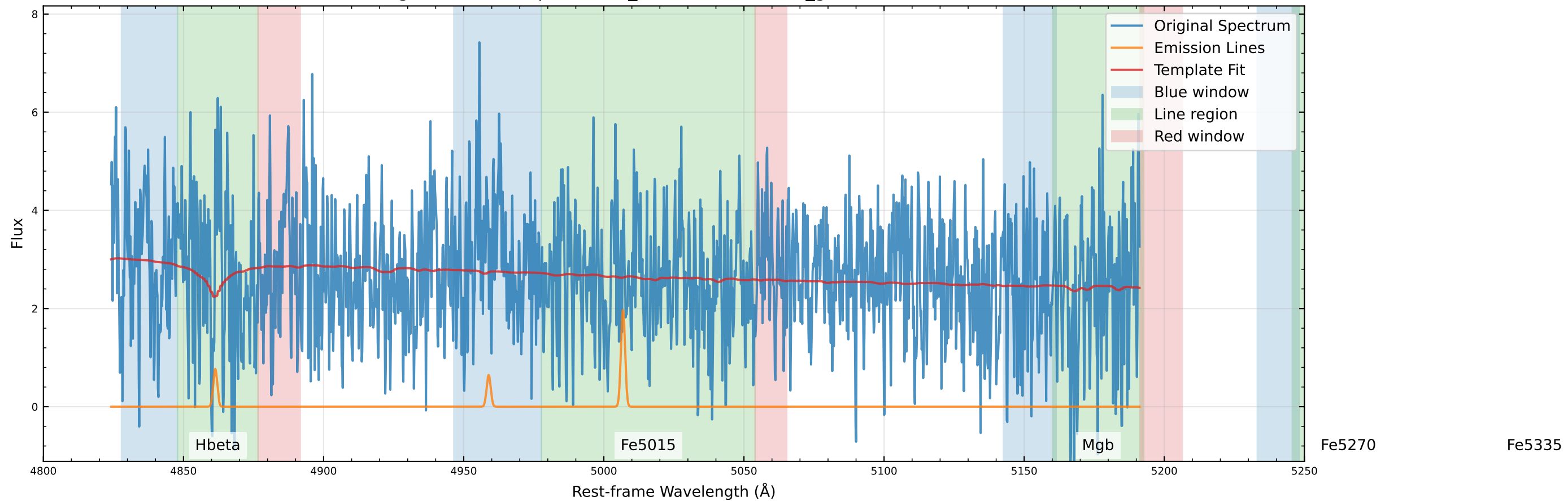
Original Data Comparison (v_star=-59.3 km/s, v_gas=-192.1 km/s)
