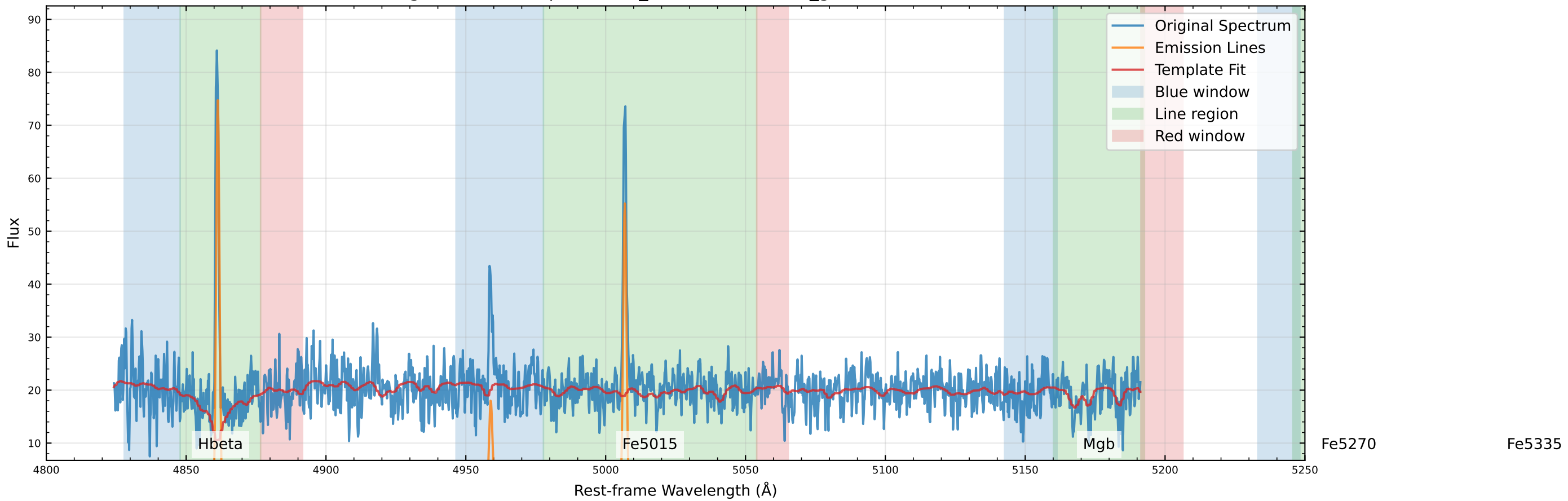
Original Data Comparison (v_star=24.9 km/s, v_gas=-10.8 km/s)
