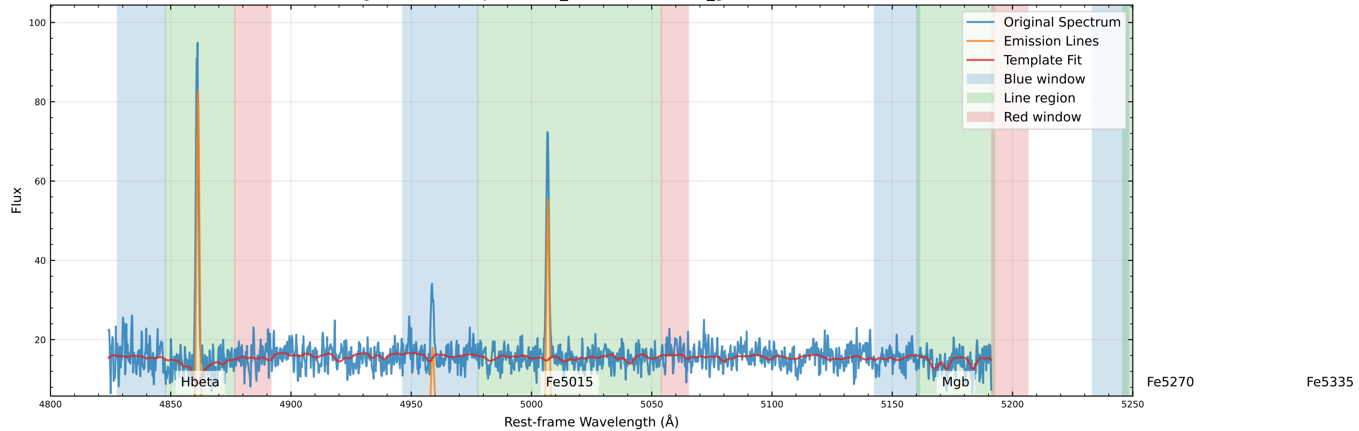
Original Data Comparison (v_star=17.3 km/s, v_gas=-16.9 km/s)
