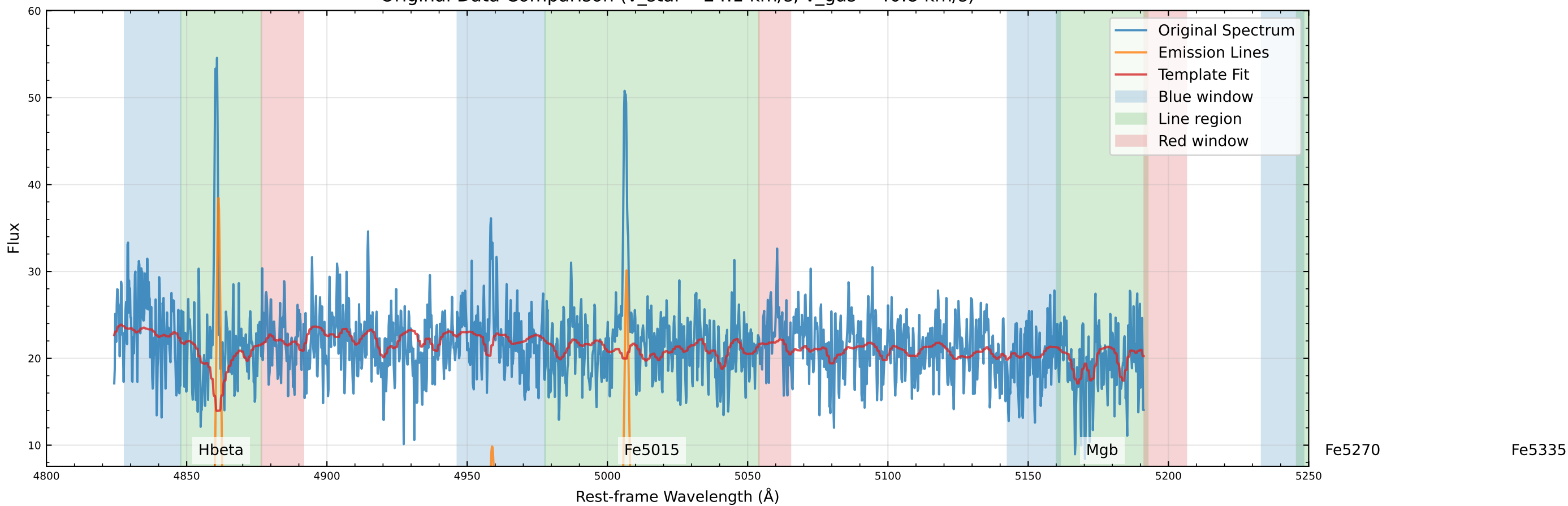
Original Data Comparison (v_star=-24.1 km/s, v_gas=-40.8 km/s)
