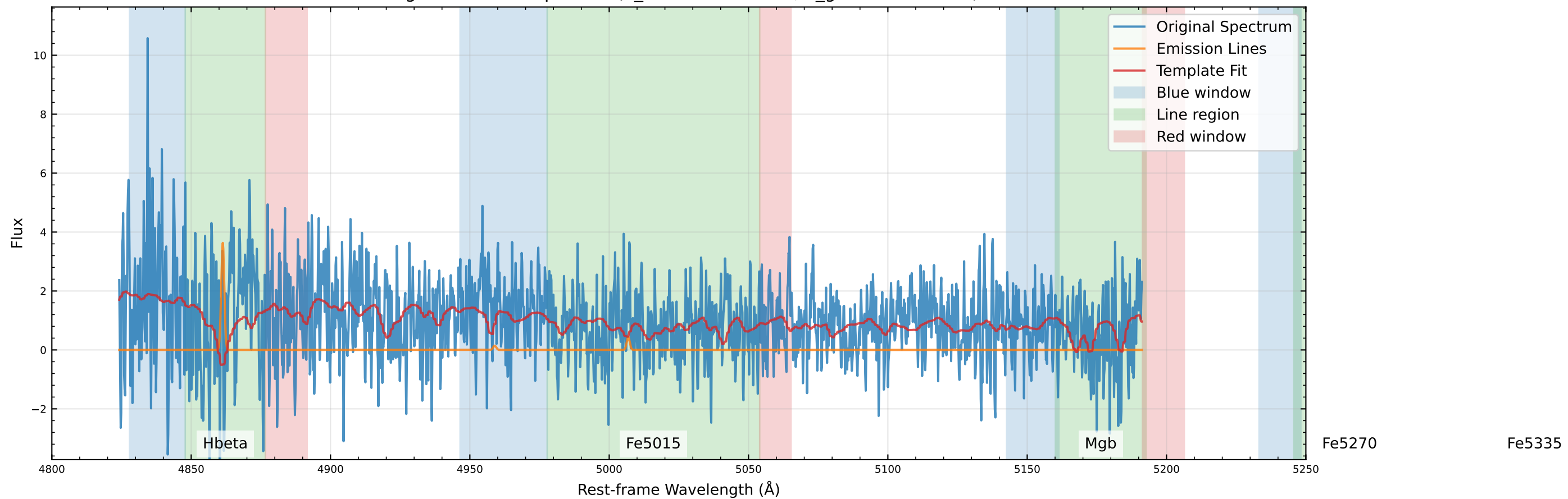
Original Data Comparison (v_star=225.3 km/s, v_gas=188.0 km/s)
