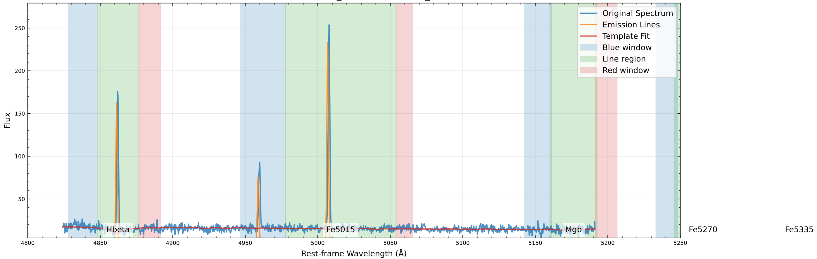
Original Data Comparison (v_star=59.4 km/s, v_gas=52.9 km/s)
