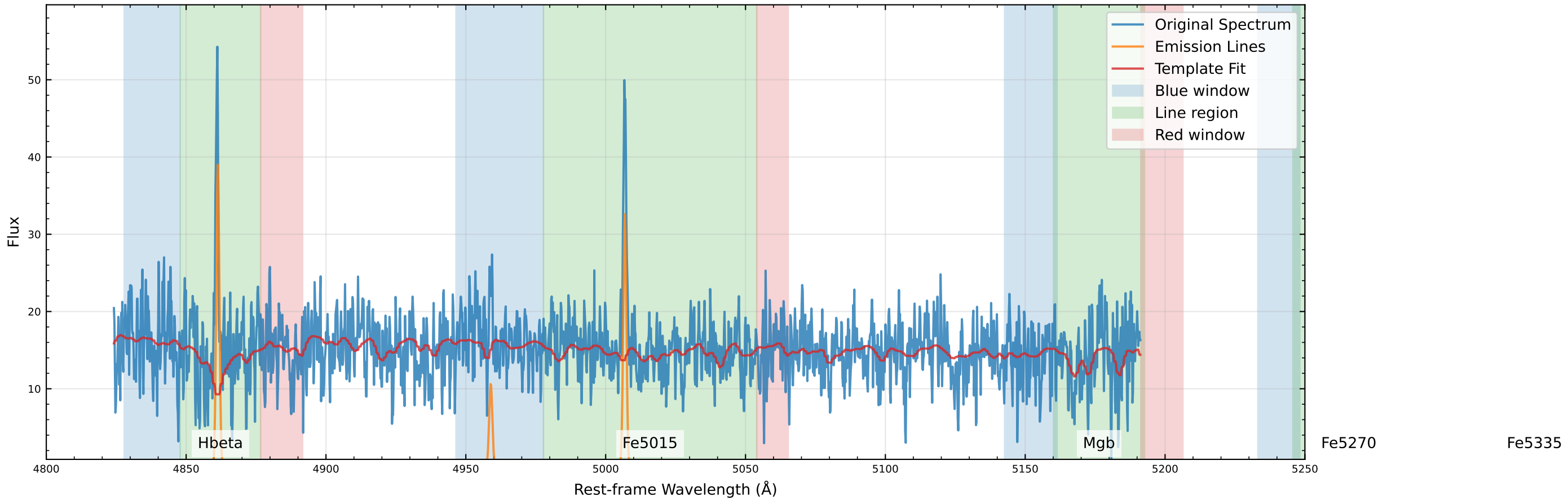
Original Data Comparison (v_star=-15.7 km/s, v_gas=-12.2 km/s)
