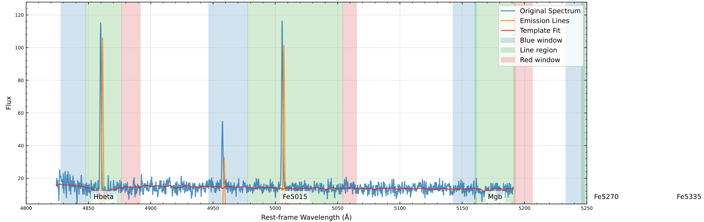
Original Data Comparison (v_star=-92.5 km/s, v_gas=-85.6 km/s)
