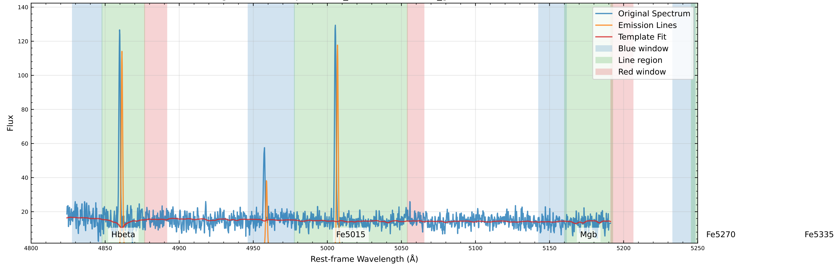
Original Data Comparison (v_star=-83.4 km/s, v_gas=-92.0 km/s)
