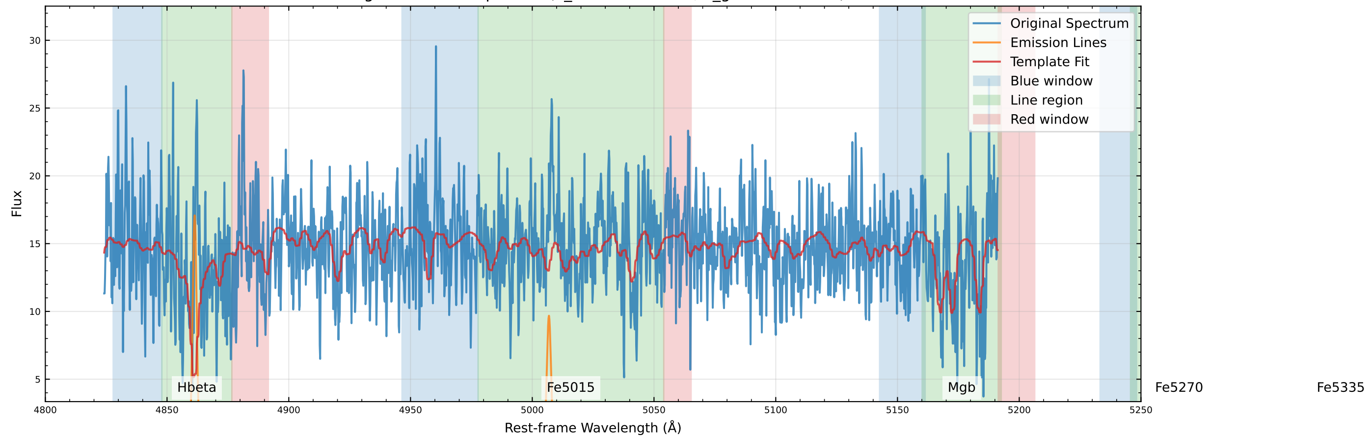
Original Data Comparison (v_star=27.0 km/s, v_gas=50.7 km/s)
