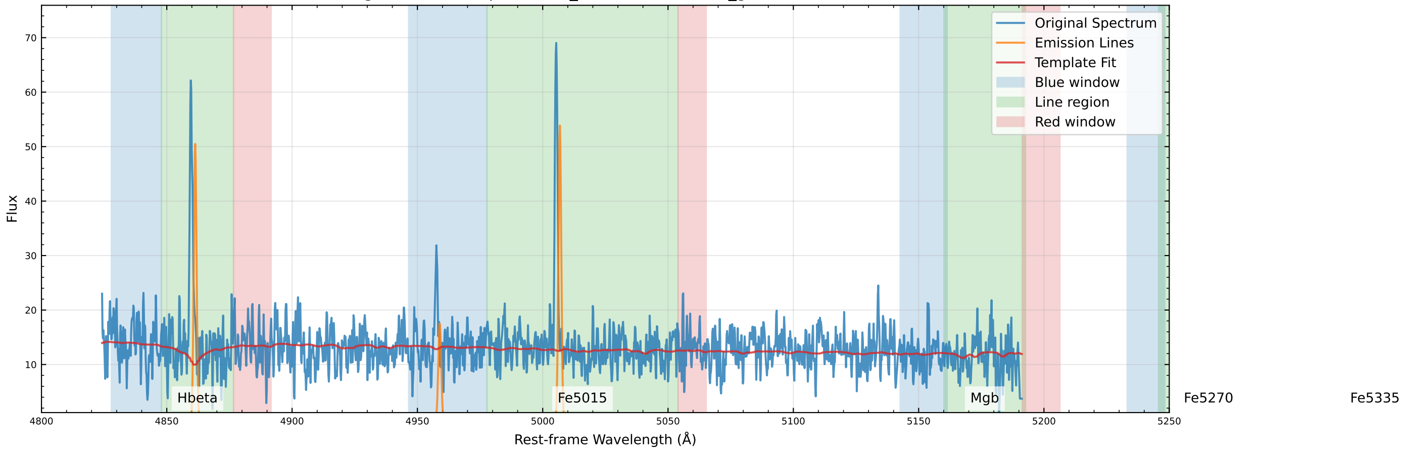
Original Data Comparison (v_star=-98.3 km/s, v_gas=-92.2 km/s)
