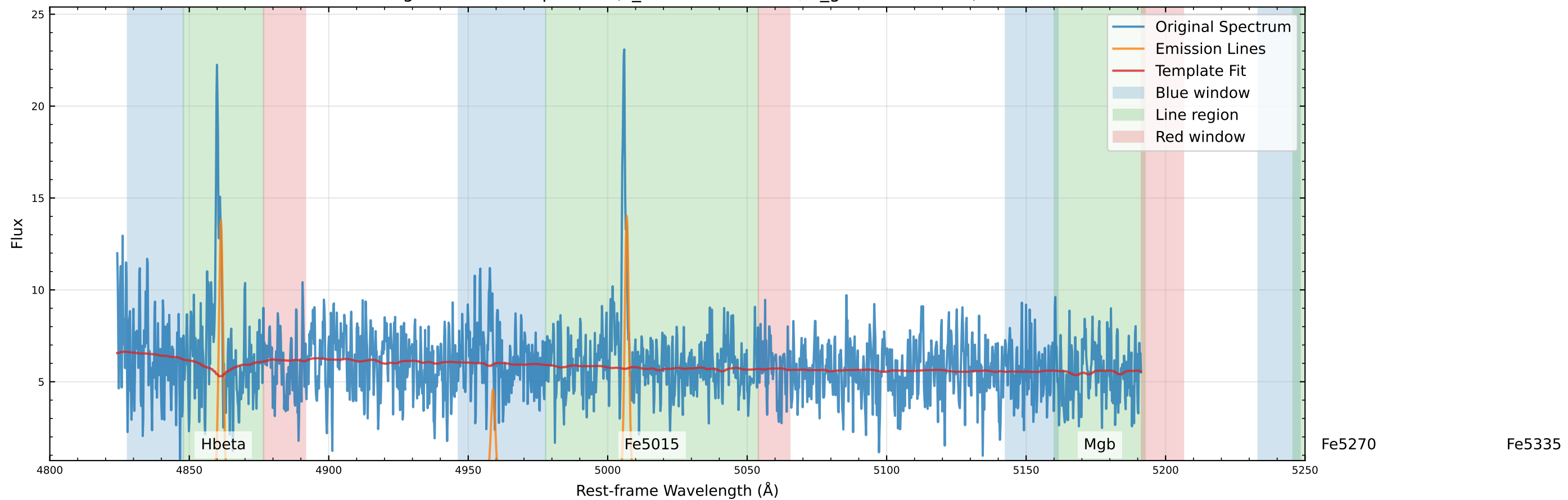
Original Data Comparison (v_star=-173.6 km/s, v_gas=-62.1 km/s)
