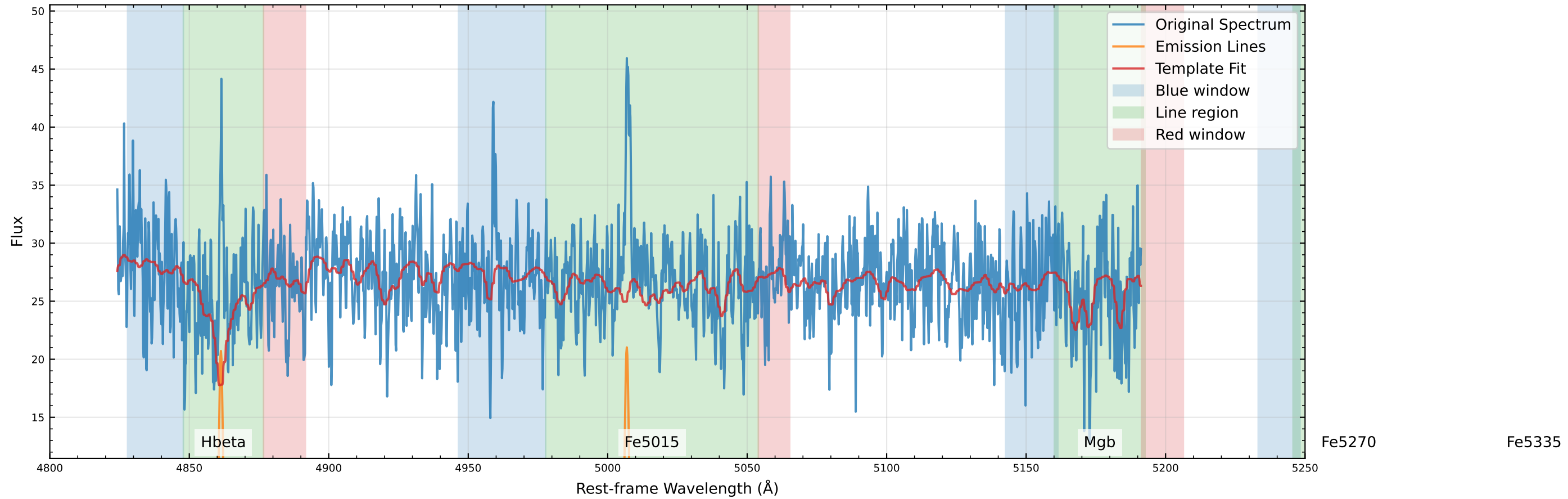
Original Data Comparison (v_star=9.2 km/s, v_gas=16.5 km/s)
