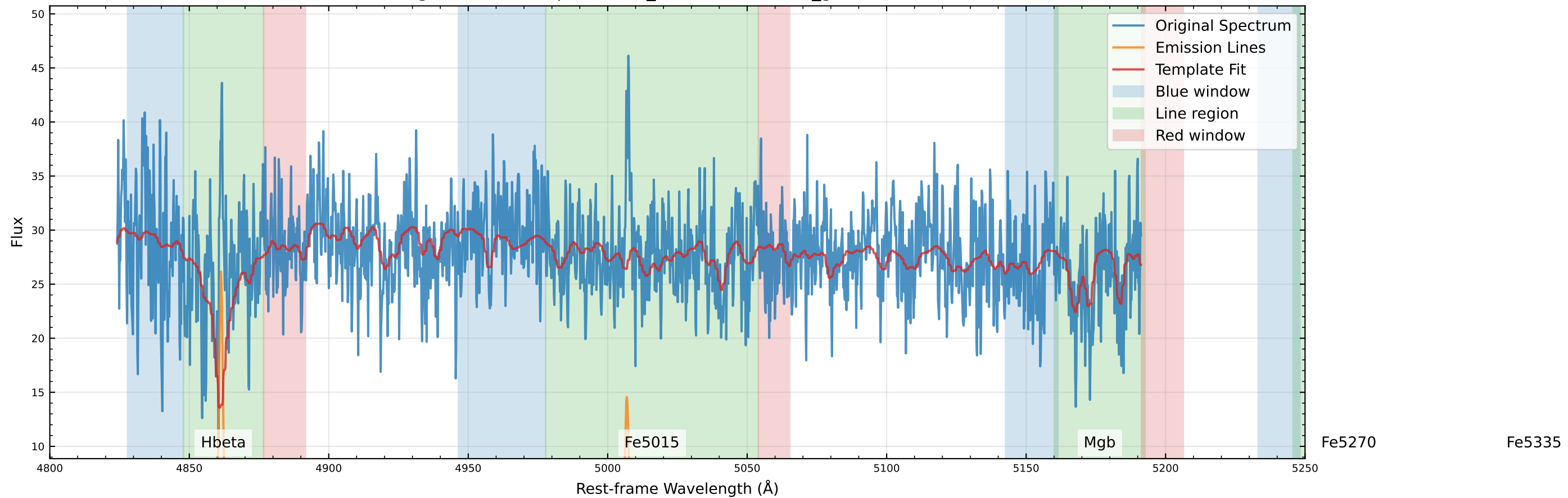
Original Data Comparison (v_star=-2.0 km/s, v_gas=16.6 km/s)
