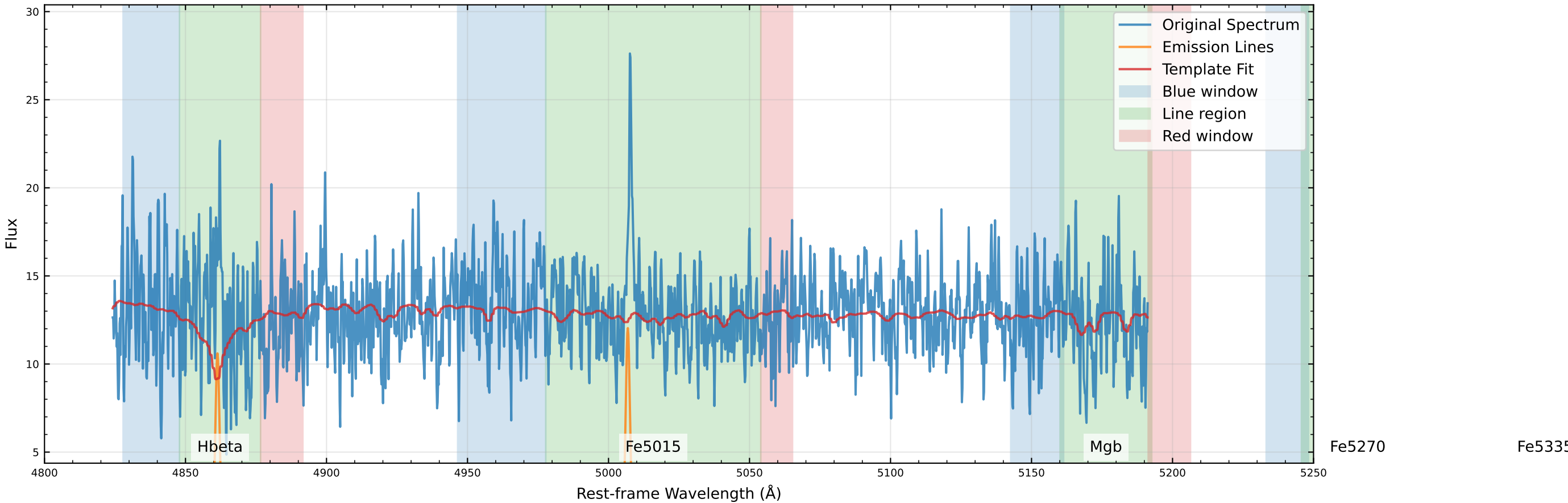
Original Data Comparison (v_star=59.8 km/s, v_gas=47.0 km/s)
