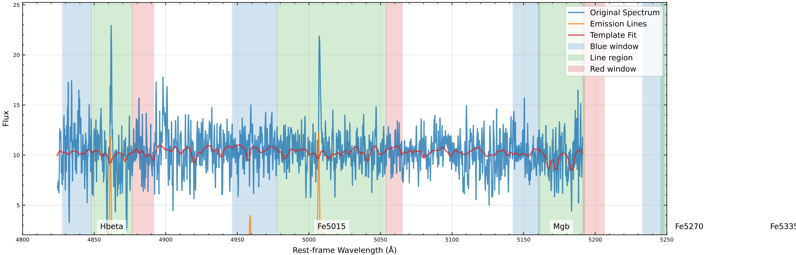
Original Data Comparison (v_star=27.5 km/s, v_gas=36.3 km/s)
