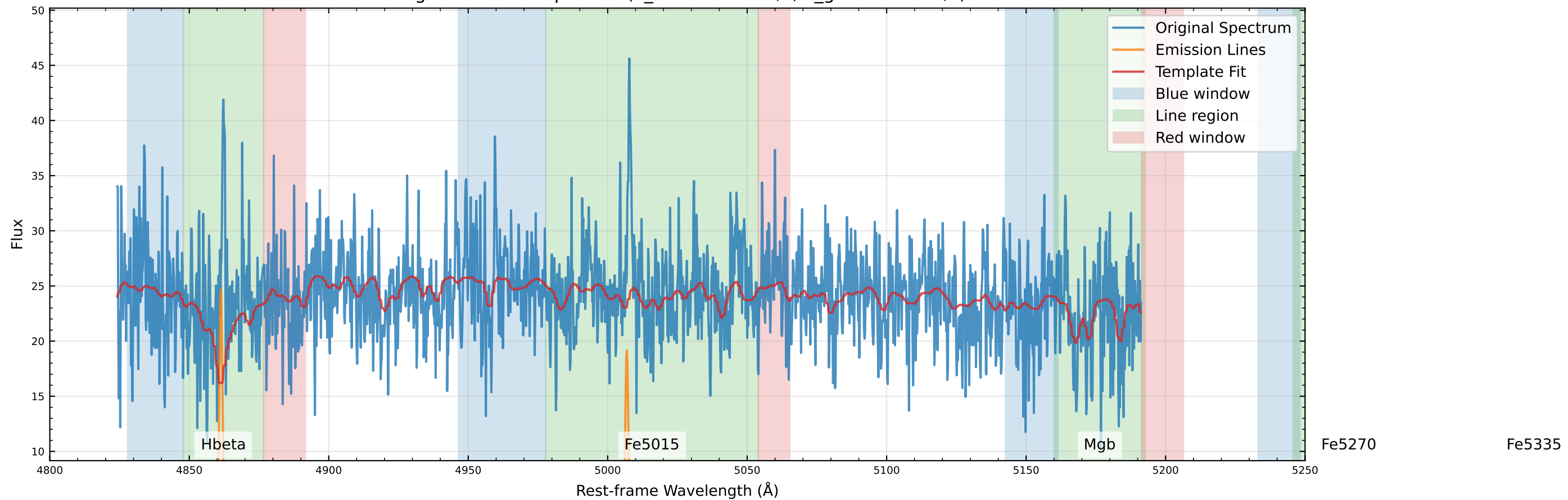
Original Data Comparison (v_star=21.0 km/s, v_gas=53.5 km/s)
