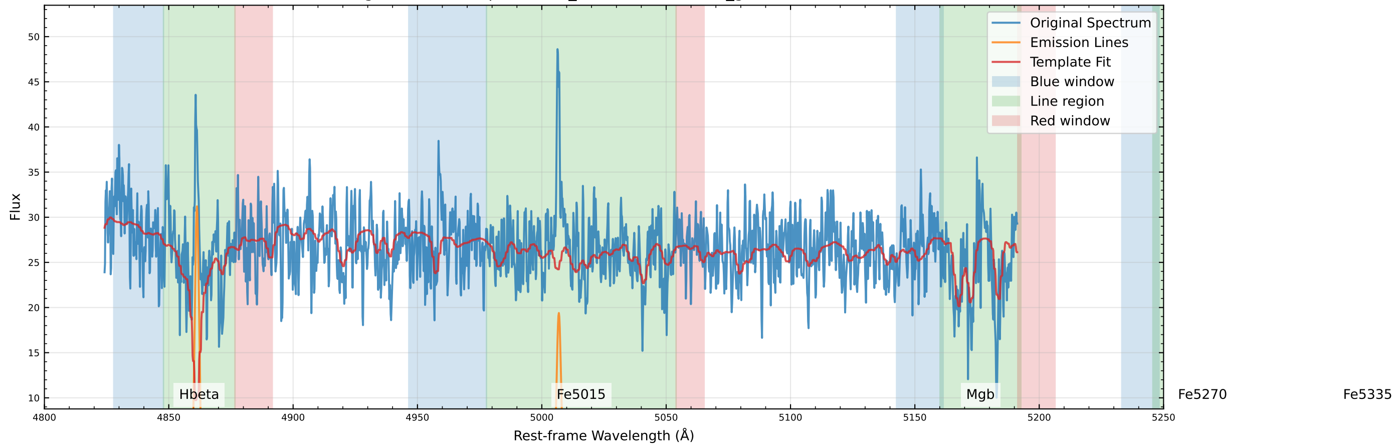
Original Data Comparison (v_star=-32.4 km/s, v_gas=-17.0 km/s)
