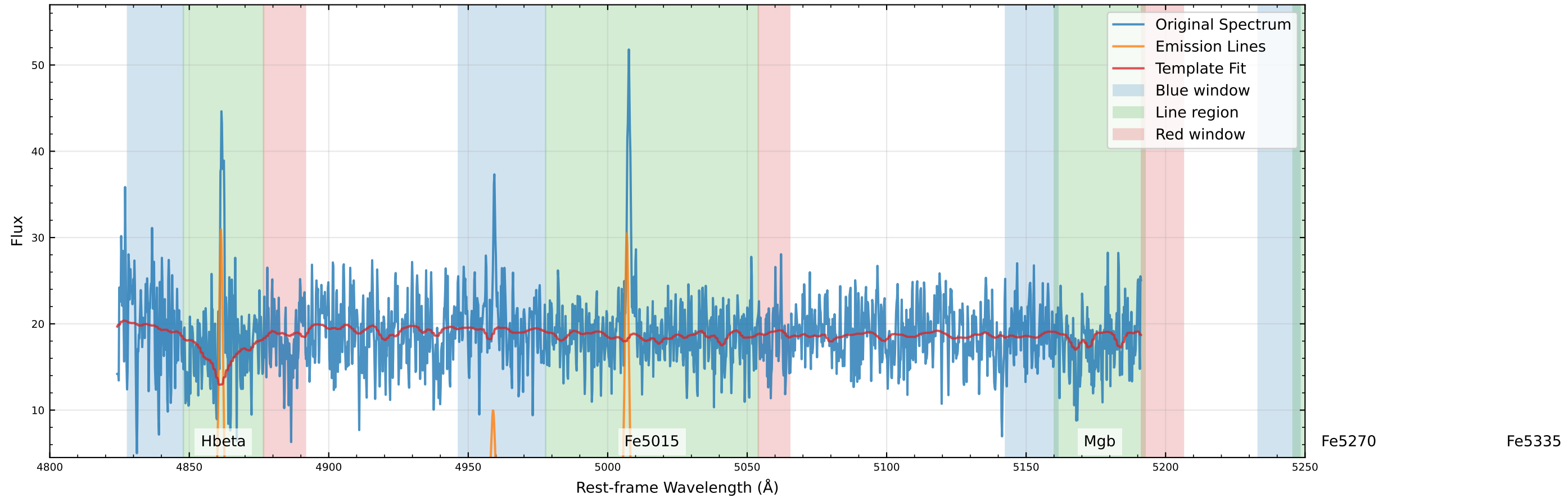
Original Data Comparison (v_star=45.9 km/s, v_gas=36.7 km/s)
