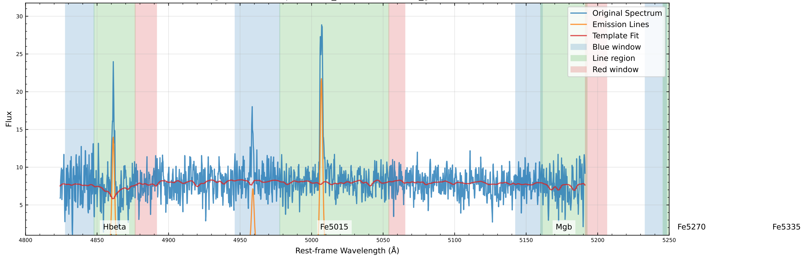
Original Data Comparison (v_star=16.0 km/s, v_gas=-0.9 km/s)
