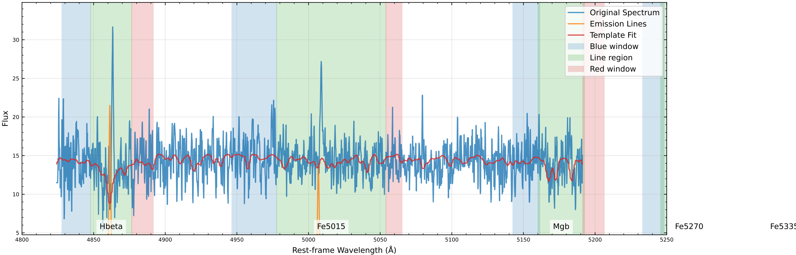
Original Data Comparison (v_star=122.3 km/s, v_gas=118.2 km/s)
