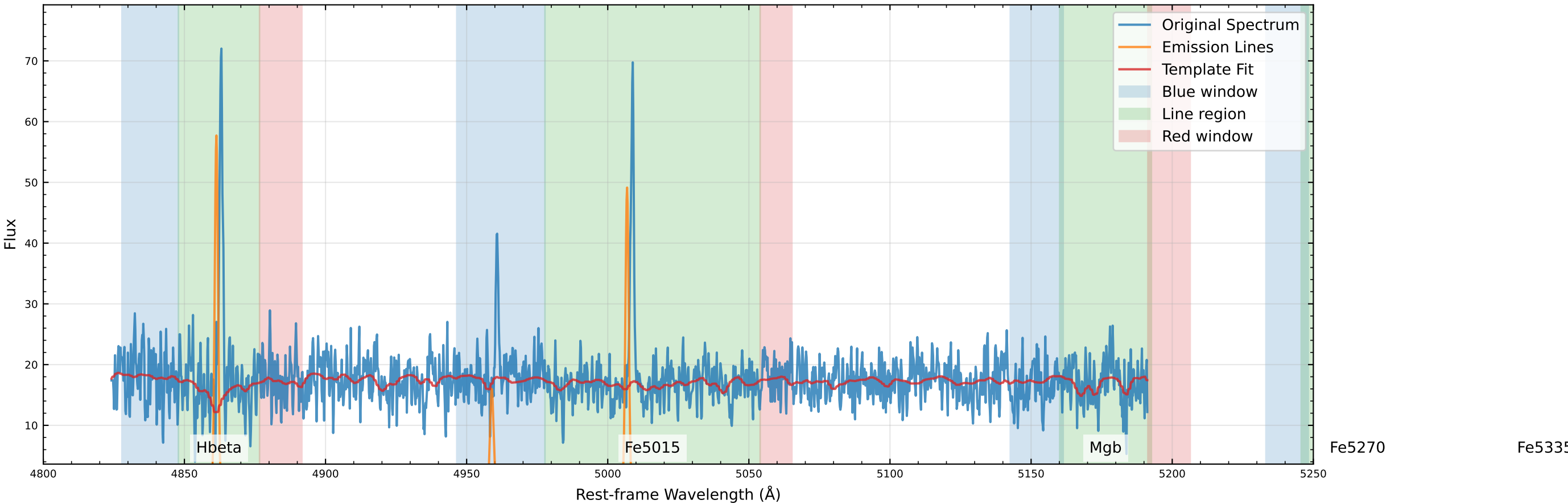
Original Data Comparison (v_star=68.3 km/s, v_gas=105.7 km/s)
