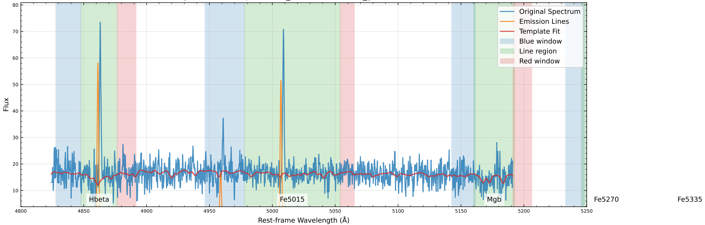
Original Data Comparison (v_star=89.1 km/s, v_gas=114.1 km/s)
