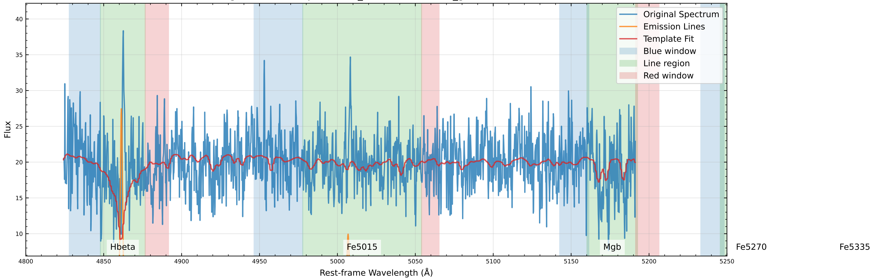
Original Data Comparison (v_star=62.4 km/s, v_gas=80.6 km/s)
